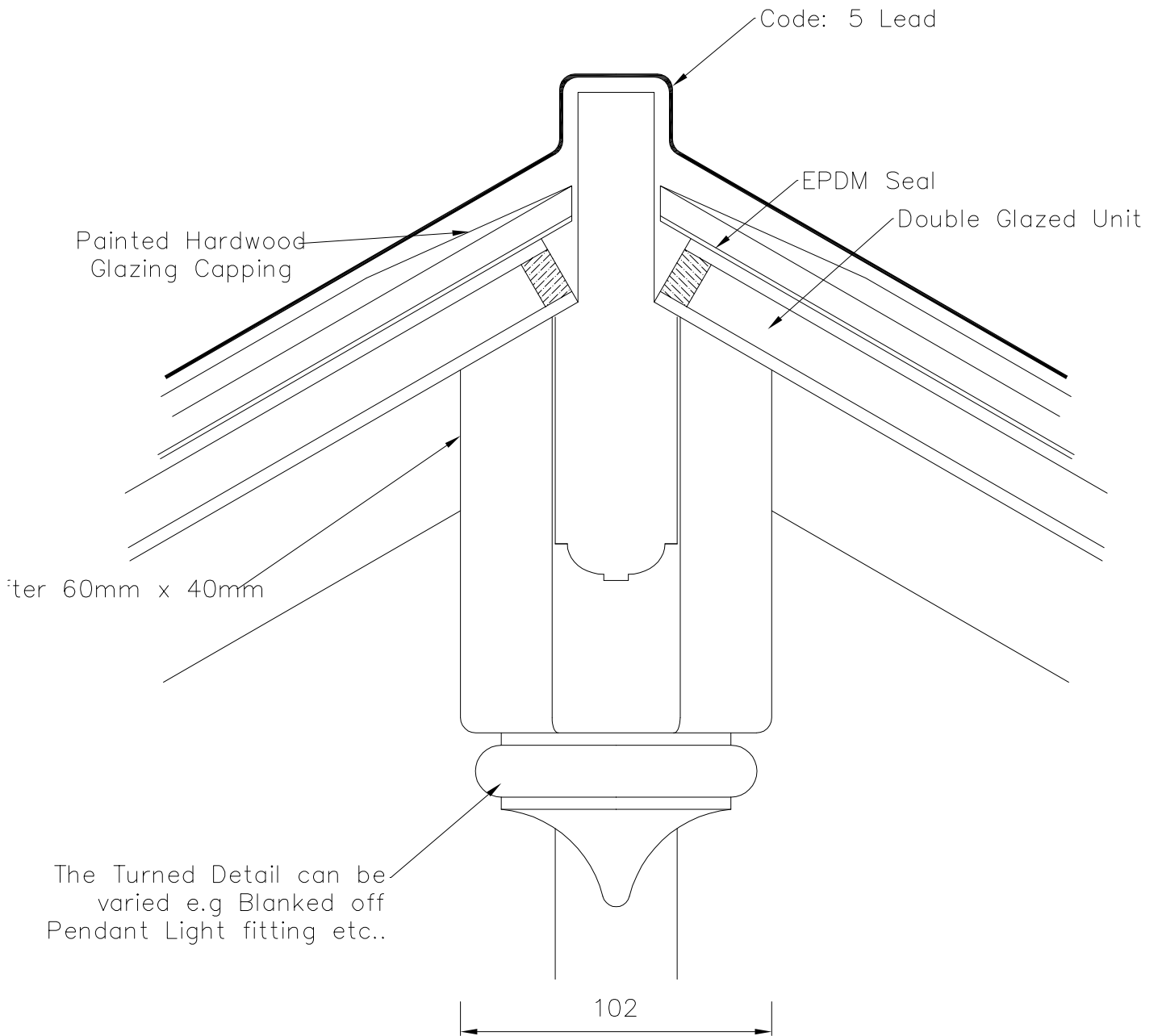
SECTION THROUGH WIDE STANDARD RIDGE (40MM)
